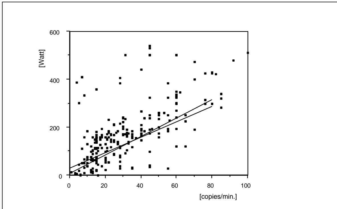
Fig. 3: Power consumption in standby mode of copiers on the market in Switzerland in 1994. The 2 lines indicate the limit for Energy Star (Tier 2) and Swiss Energie 2000 Label. (Most of the copiers with a capacity of more than 20 copies/min and a power consumption much below the two lines have a recovery time exceeding 30 seconds)
