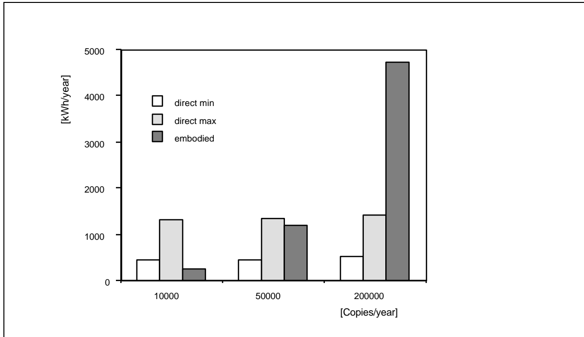
Fig. 2: Annual consumption of direct and (in paper) embodied energy of a typical copier with a copying capacity of 40 copies per minute (own calculation)
