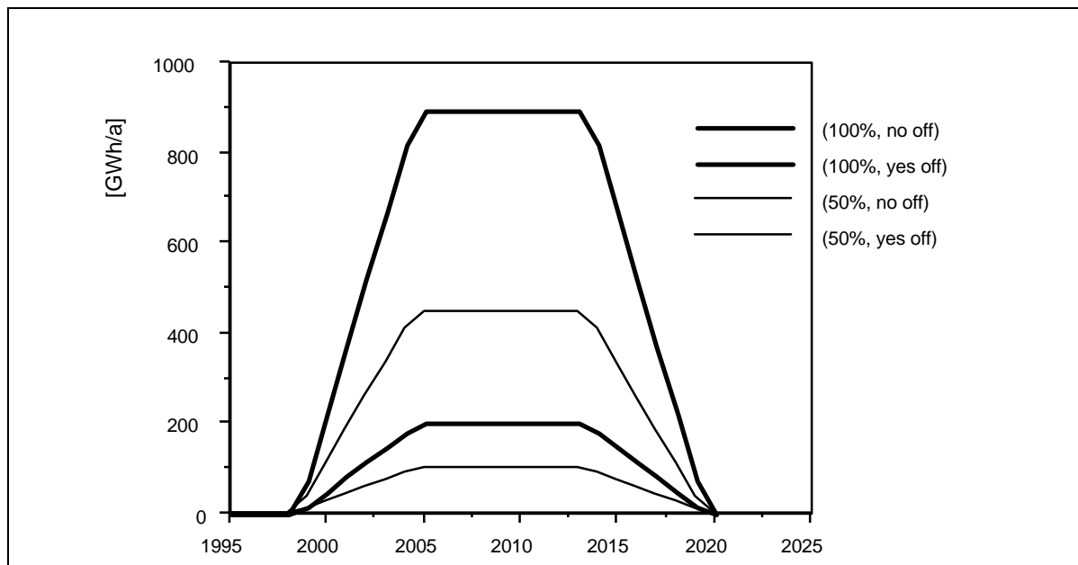
Fig. 1: Annual energy saving if the innovative copier is introduced on the market two years earlier than in the reference case (without procurement). The lines shown in the figure differ by two parameters (a, b), e. g. (100%, no off) for the first line. "a" designs the supposed market penetration of the innovative copier (with and without accelerated introduction) in the year 2015 and "b" describes whether the copier with traditional technology is turned off (or not turned off) during non-working hours [own calculation].
