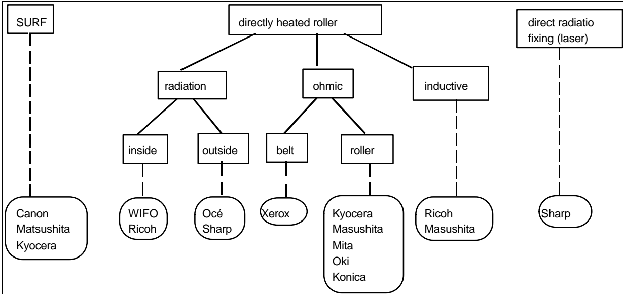
Fig. 4: Genealogy of patents related to low energy standby mode fixing [Jea 1996, Rep. 2, Fig. 1]
